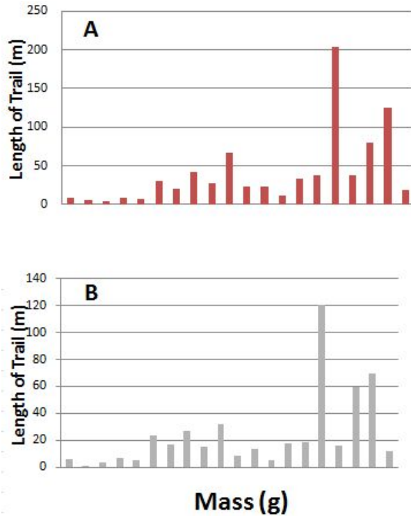
FIGURE 3. Length of fluorescent powder trails left by three species of garter snakes (10 Thamnophis sirtalis , five T. radix , one T. elegans , and three snakes lacking species records [likely T. sirtalis ]). Individuals' performances are organized along the X axis left to right based on increasing body size, smallest mass (3.1 g) to largest mass (171.6 g) of snake. Actual distance (A) is the sum of distances measured between turns of 10 or more degrees. Straight line distance (B) is the linear distance from the point where the snake was released to the point where powder was last detected.
